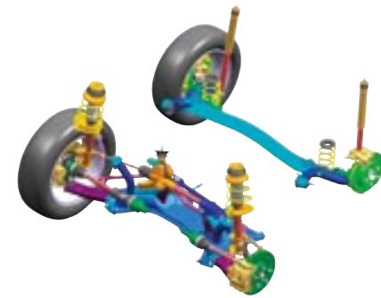
Suspension System. An independent MacPherson strut front suspension is teamed with a highly rigid torsion-beam setup in the rear, providing responsive, linear handling, and stable cornering performance.
